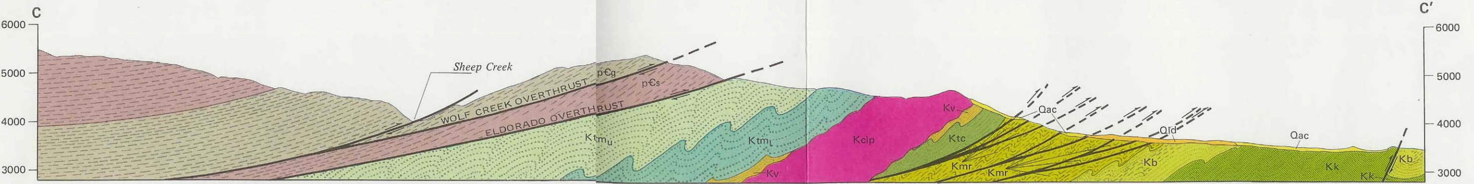
Section C-C'
