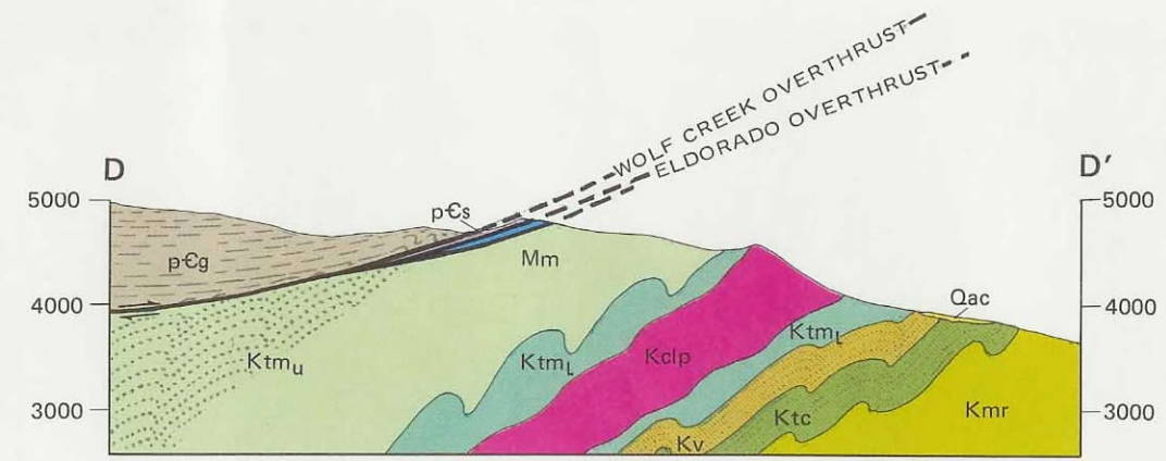
Section D-D'
